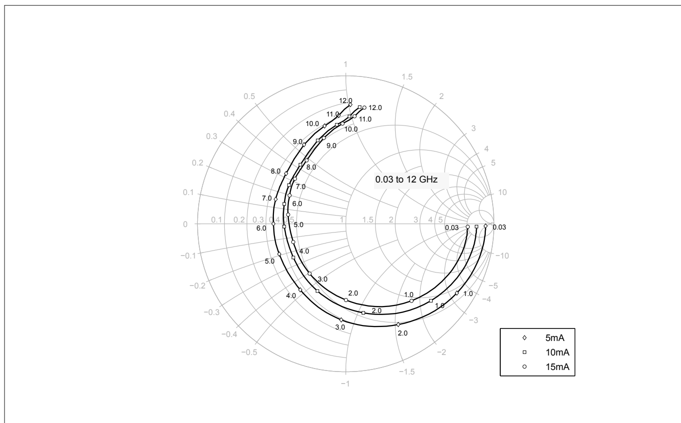
Figure 16 Input reflection coefficient S_{11} = f(f) , V_{CE} = 1.8 \text{ V} , I_C = 5 / 10 / 15 \text{ mA}
