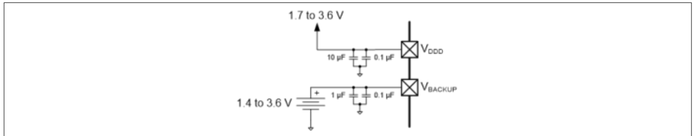
Figure 17 Separate Battery Connection to V_{BACKUP}
