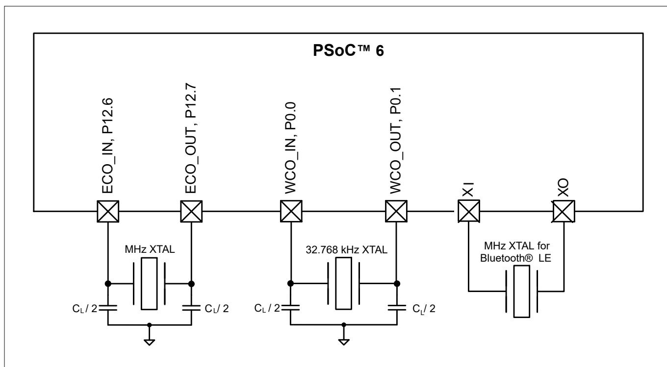
Figure 5 Oscillator circuits
