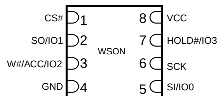
Figure 4. 8-contact WSON Package (6 x 8 mm)
