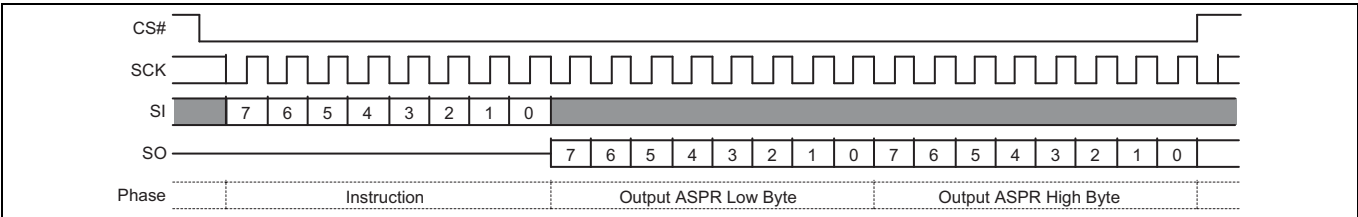
Figure 102 ASPRD command
