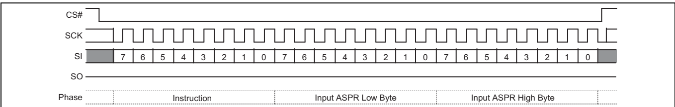
Figure 103 ASPP command
