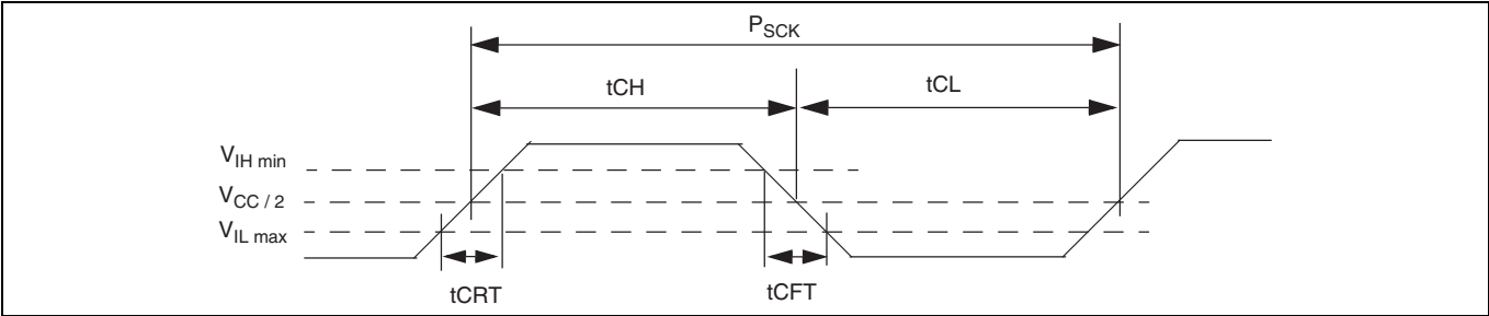
Figure 28 Clock timing
