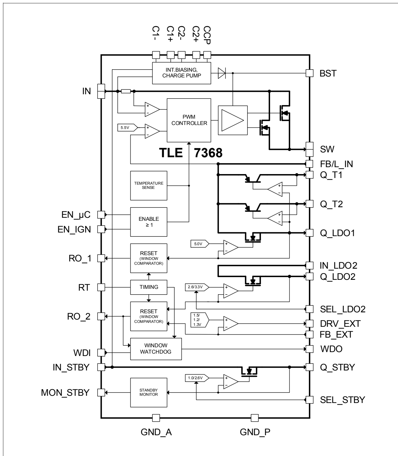
Figure 1 Block Diagram
