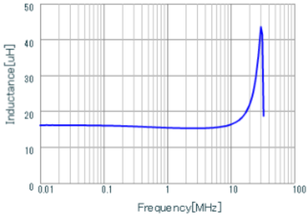
LQH2HPN150MJR L
