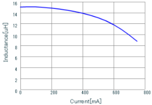
LQH2HPN150MJR DC-Bias, 20
