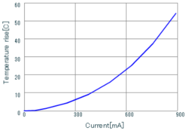
LQH2HPN150MJR DT_Current
