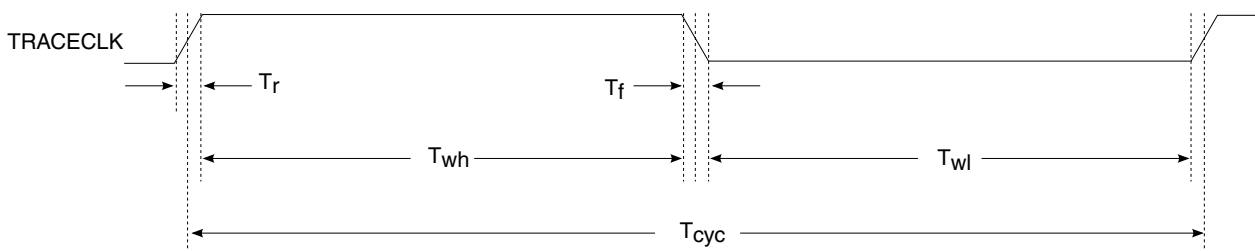
Figure 5. TRACE_CLKOUT specifications
