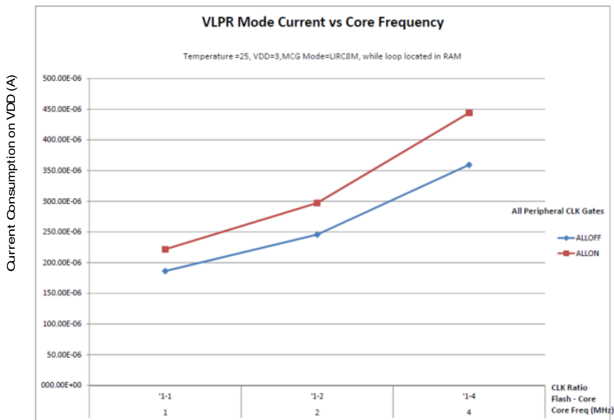
Figure 18. VLPR mode current vs. core frequency
