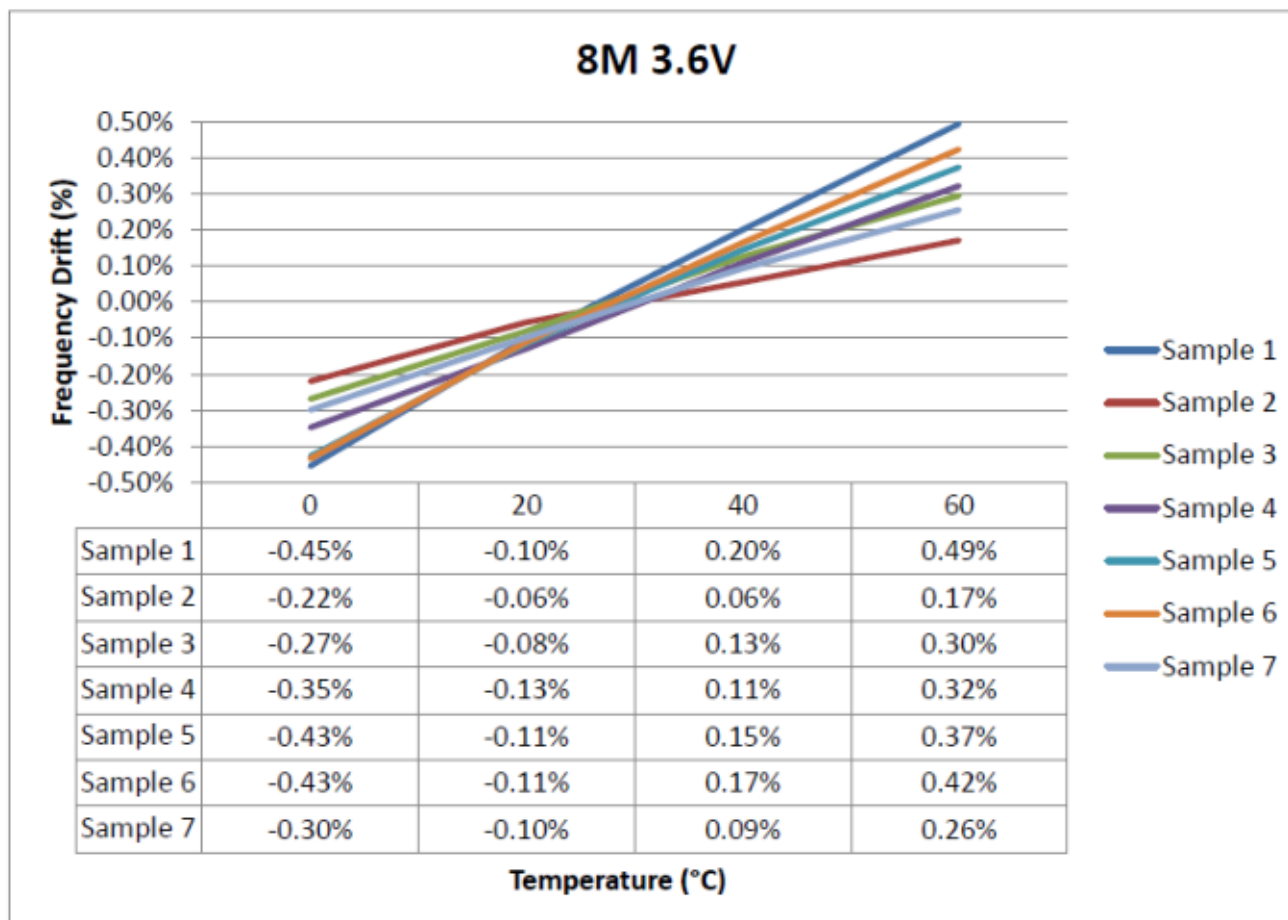
Figure 21. IRC8M Frequency Drift vs Temperature curve
