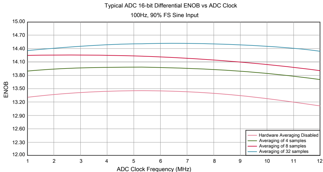
Figure 23. Typical ENOB vs. ADC_CLK for 16-bit differential mode
