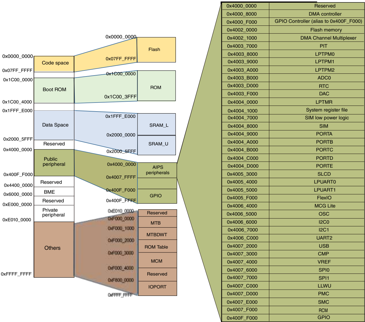
Figure 4. Memory map
