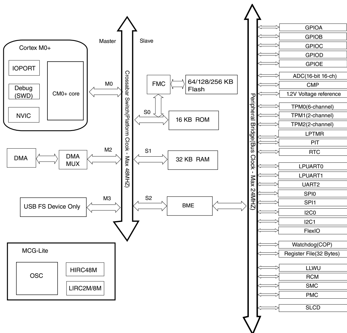
Figure 1. System diagram
