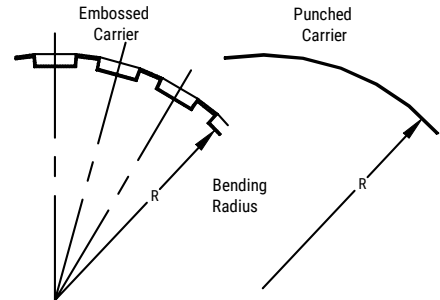
Figure 4 – Bending Radius
