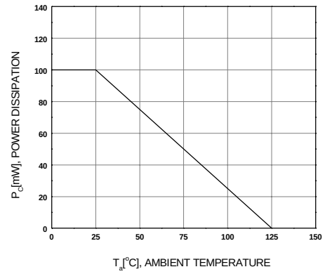
Figure 8. P_D - T_A
