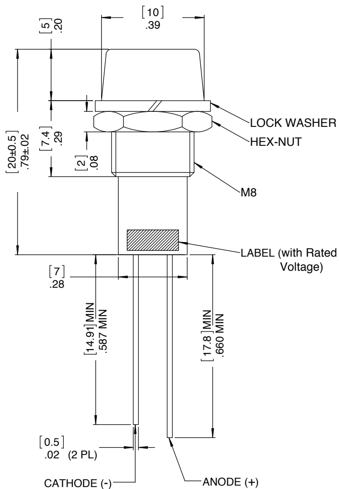
L65DX12L L65DX24L
