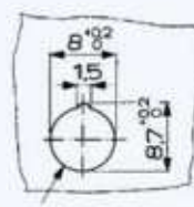
Front panel drilling
