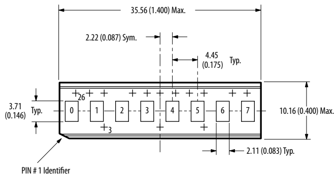
HCMS-291x/HCMS-391x
