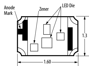
HSMF-C129
