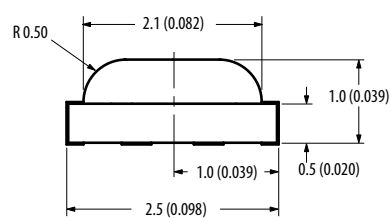
HSMF-C113/C115
