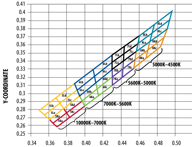
Color Bin Selection ( X_1 ) for ASMT-QYBx
