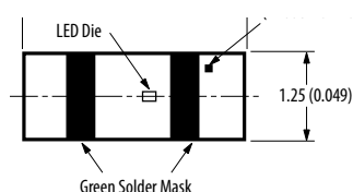
HSMx-C265
