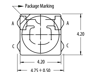
Package Drawing C
