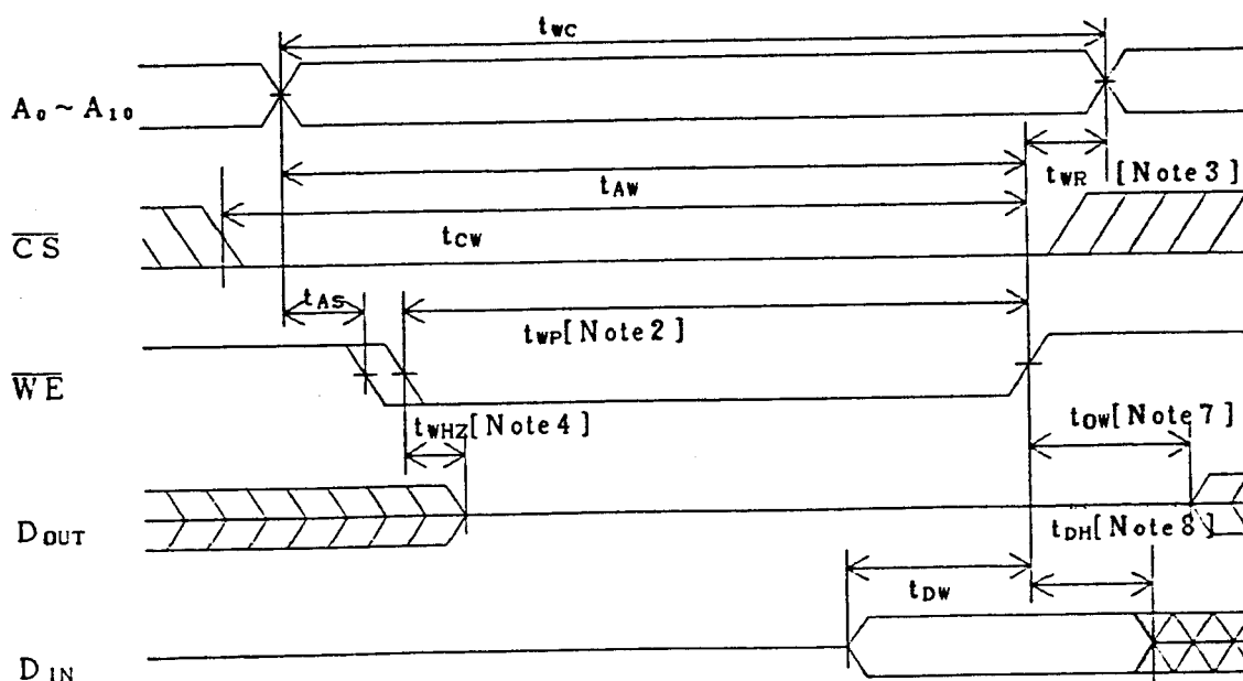
Timing Chart(No.1)[Note1,6]
