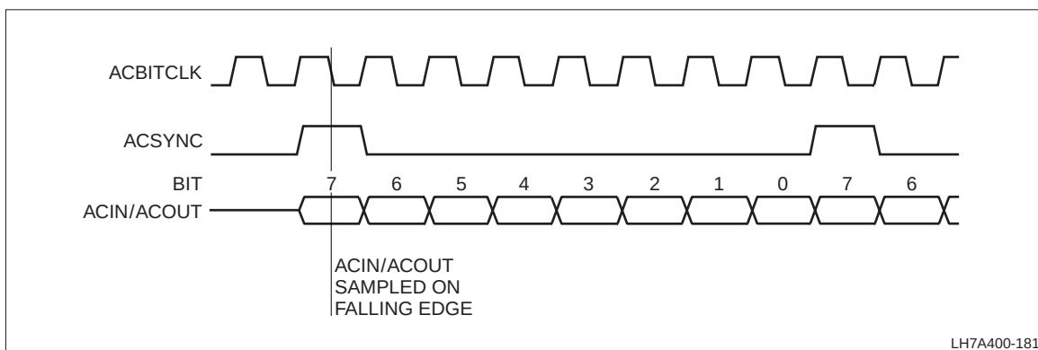
Figure 20. ACI Datastream
