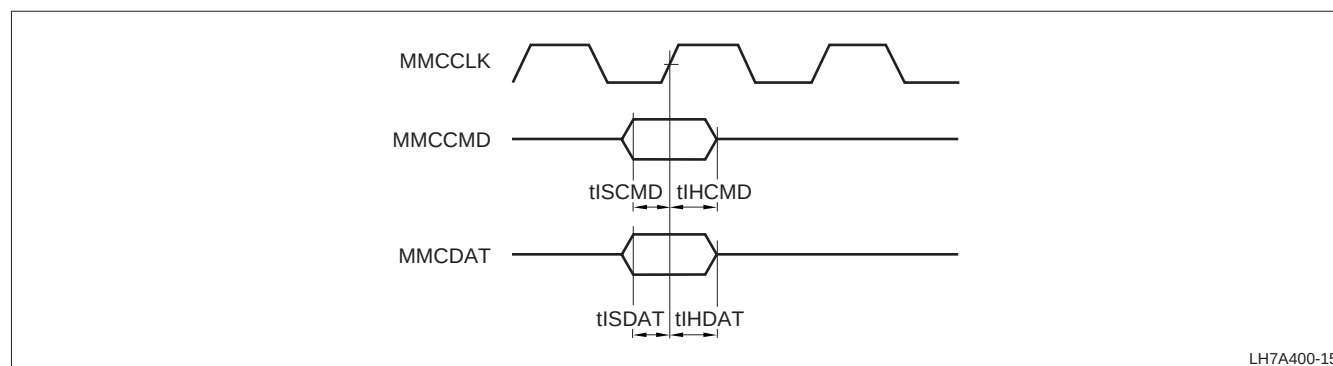
Figure 17. MMC Command/Data Read
