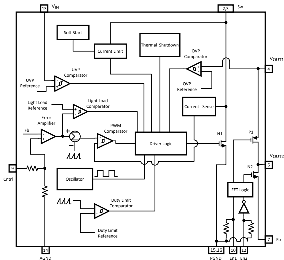
Figure 3. Block Diagram
