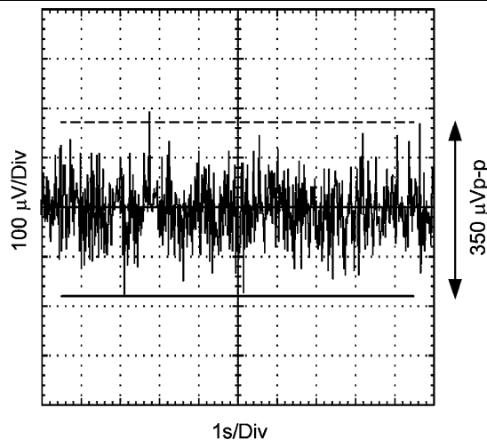
Figure 44. 0.1–10 Hz Noise
