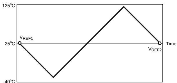
Figure 47. Temperature Profile
