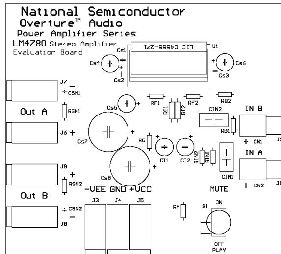
Figure 41. Silk Layer
