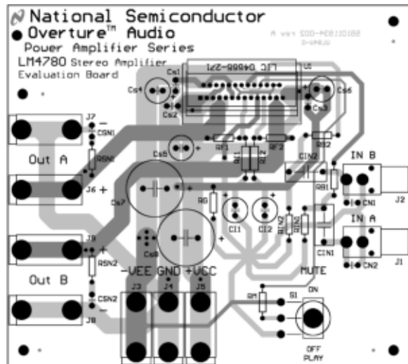
Figure 40. Composite Layer
