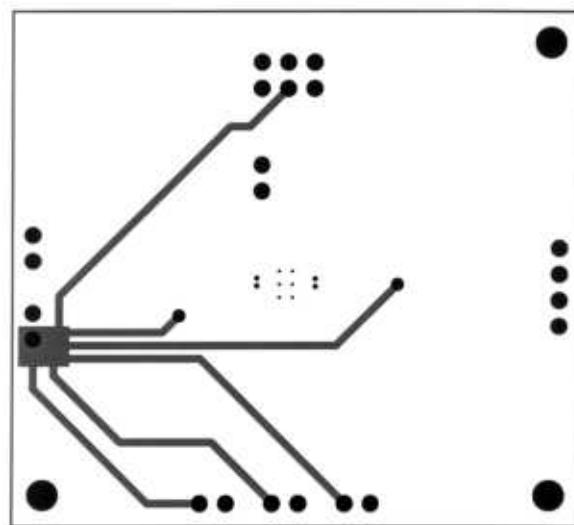
Figure 49. Recommended LQ PC Board Layout: Inner Layer 2
