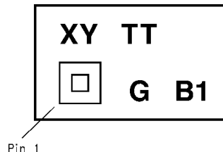
Figure 3. 18-Bump micro SMD Marking (ITL) (Top View) XY- Date Code TT - Die Traceability G - Boomer Family B1 - LM4851ITL
