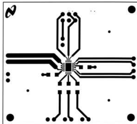
Figure 47. Recommended LQ PC Board Layout: Top Layer
