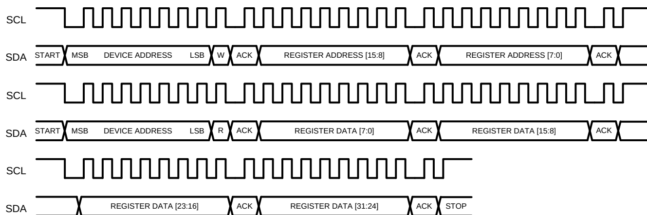
Figure 9. Example I 2 C Read Sequence
