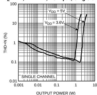
THD+N vs OUTPUT POWER R_L = 4\Omega , f = 1\text{kHz} , I 2 S Input, Single channel
