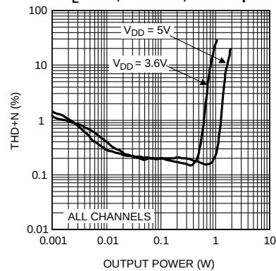
THD+N vs OUTPUT POWER R_L = 4\Omega , f = 1\text{kHz} , ADC Input, Parallel mode
