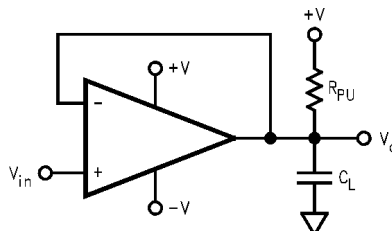
Figure 52. Using a Pull-Up Resistor at the Output for Stabilizing Capacitive Loads
