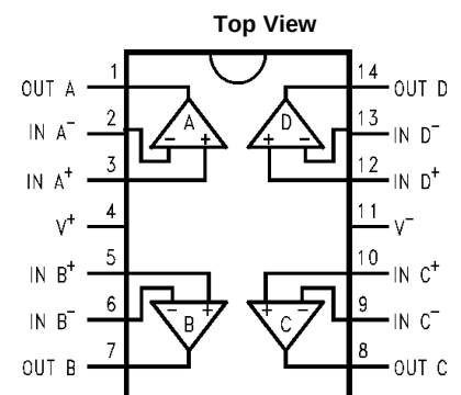
Figure 61. 14-Pin TSSOP/SOIC Package
