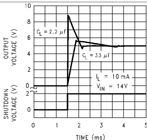
Figure 16. Enable Transient
