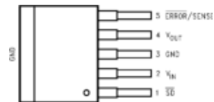
Figure 2. Top View 5-Pin DDPAK/TO-263 See KTT0005B Package
