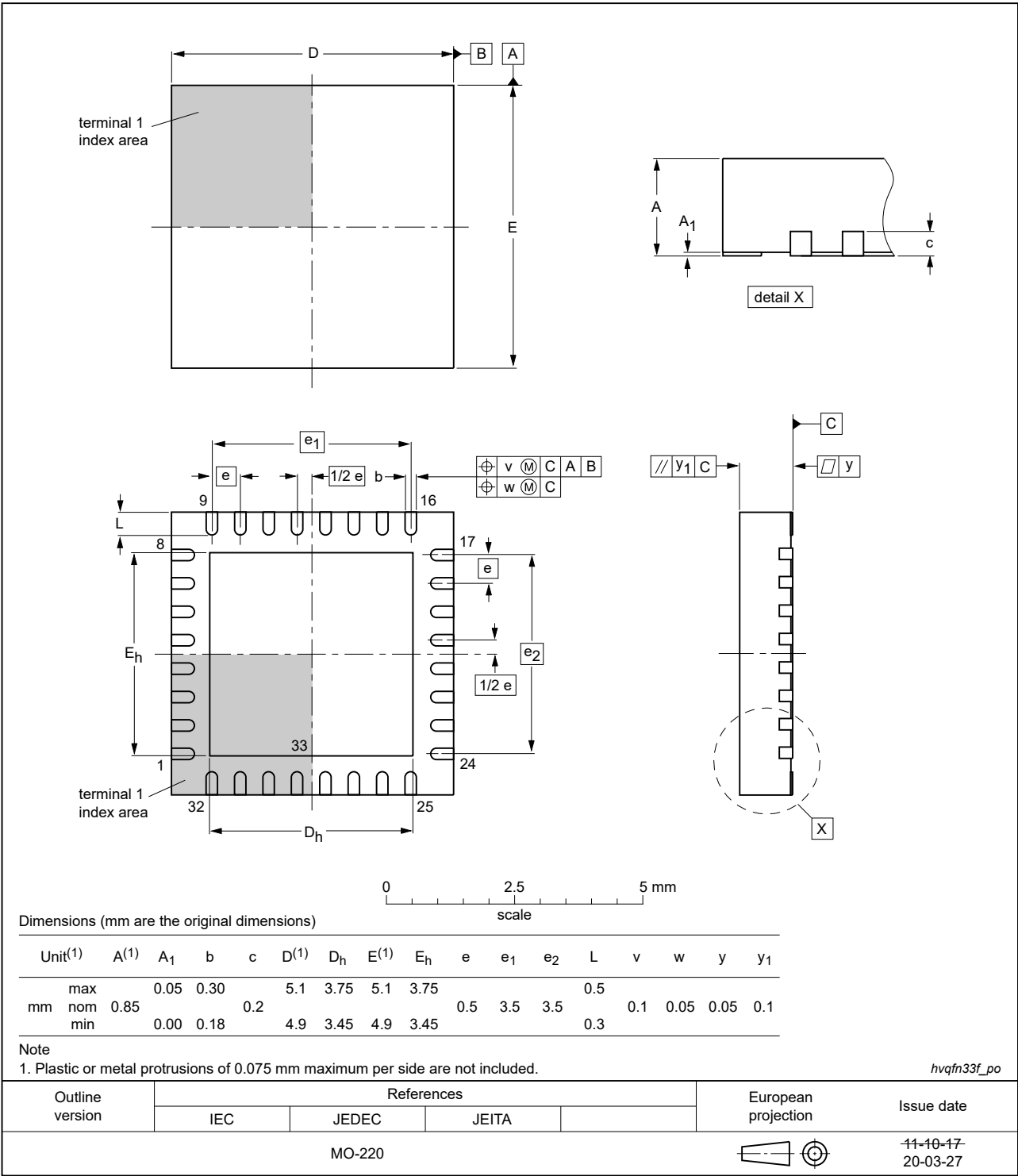
Figure 34. Package outline HVQFN33 (5 x 5 x 0.85 mm)
