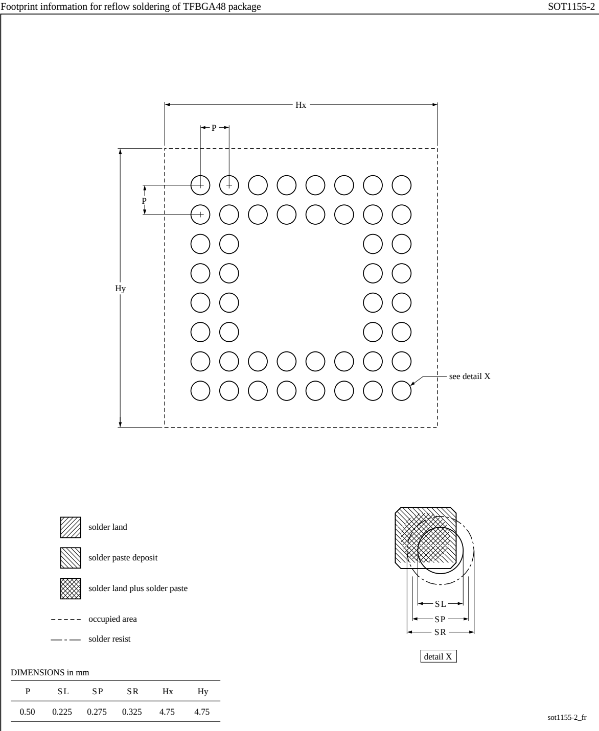
Figure 41. Reflow soldering for the TFBGA48 package
