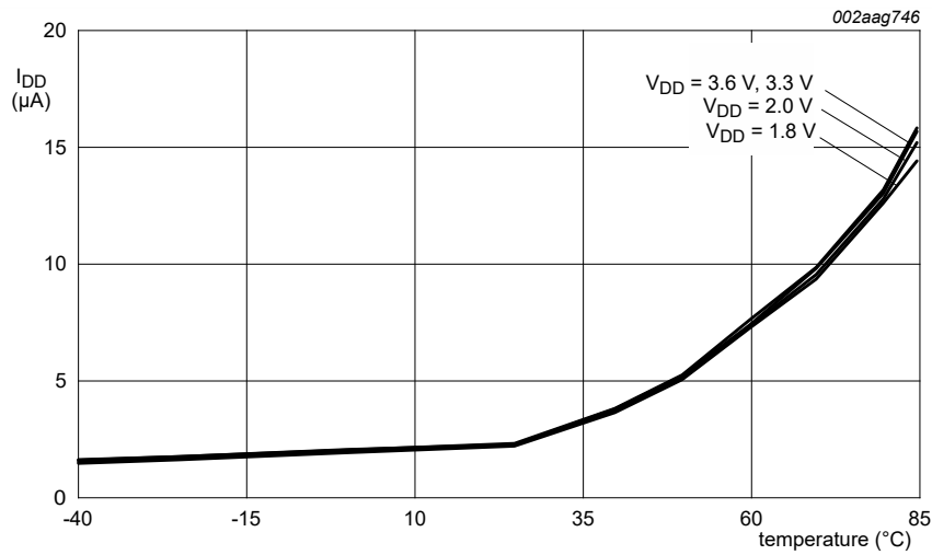
Figure 13. Typical supply current versus temperature in Power-down mode
