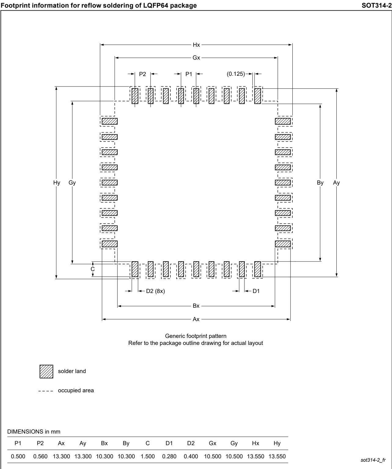
Figure 43. Reflow soldering for the LQFP64 package
