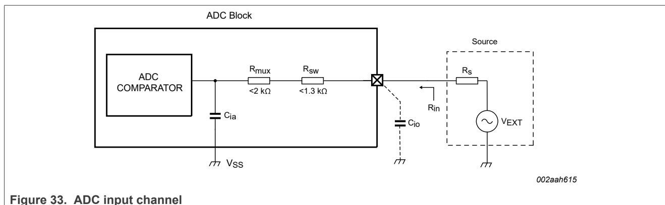
Figure 33. ADC input channel
