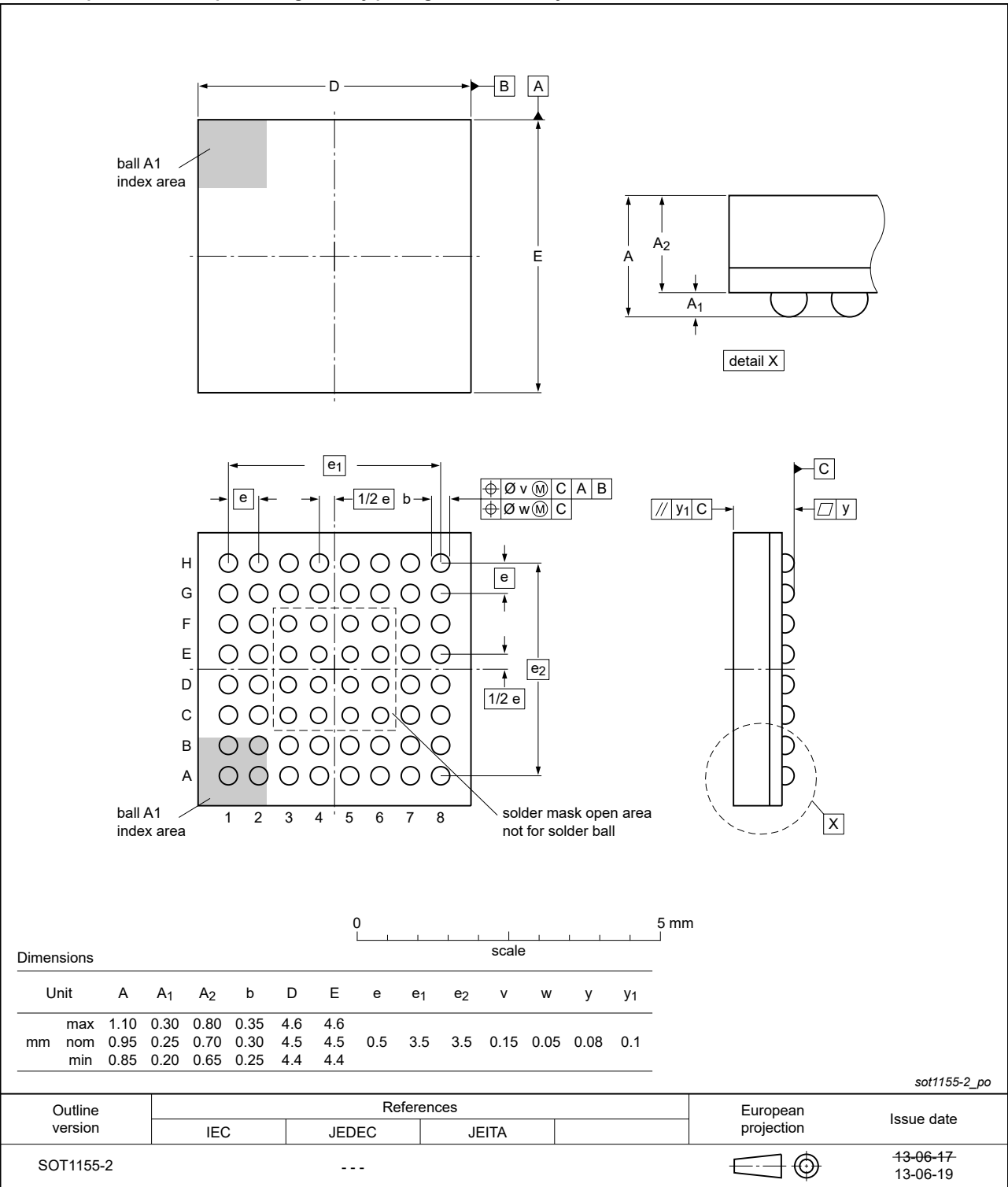
Figure 36. Package outline TFBGA48 (SOT1155-2)
