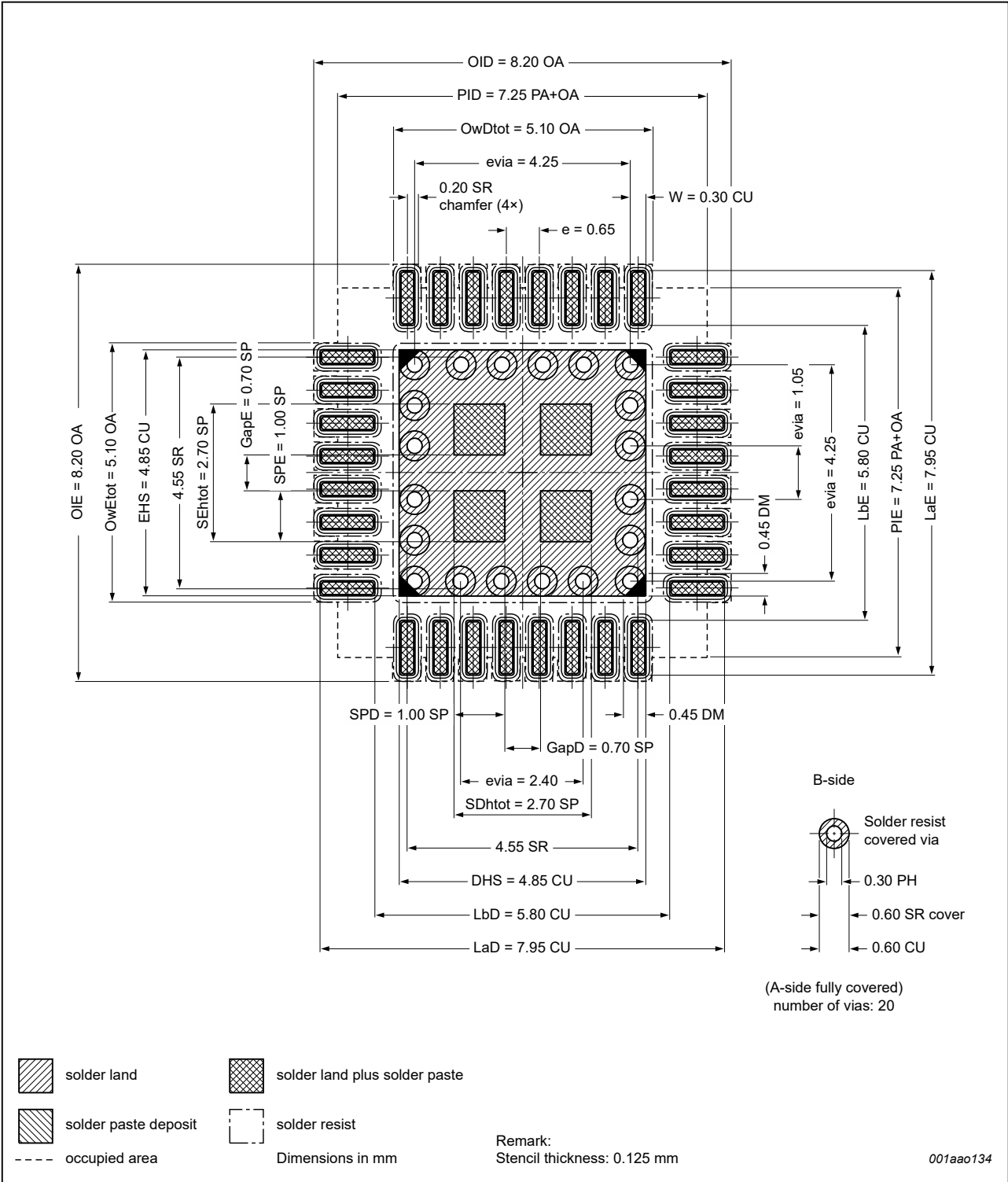
Figure 40. Reflow soldering for the HVQFN33 (7x7) package
