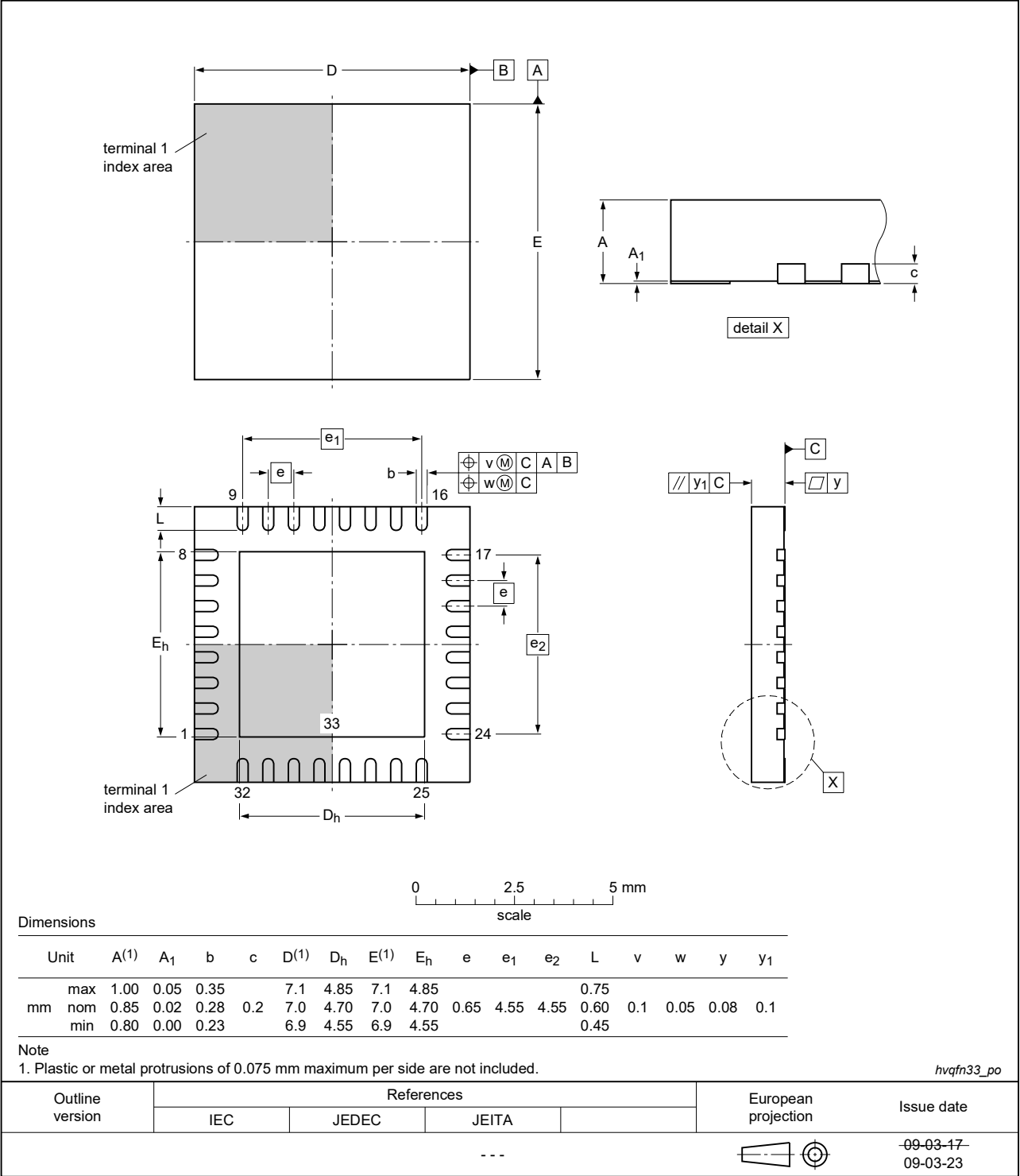
Figure 35. Package outline HVQFN33 (7 x 7 x 0.85 mm)
