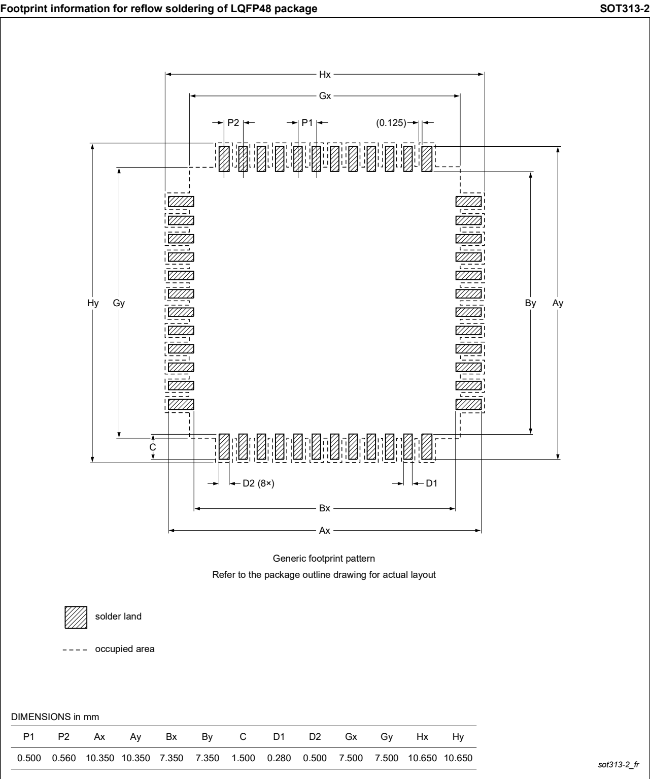
Figure 42. Reflow soldering for the LQFP48 package
