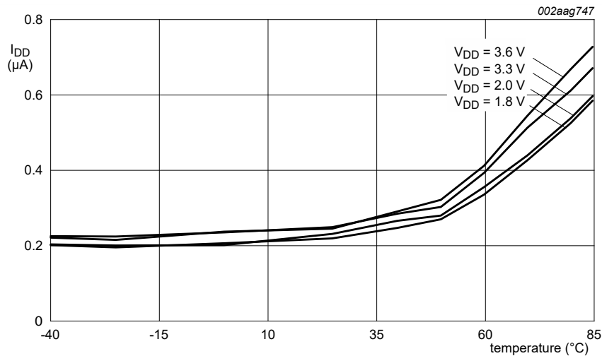
Figure 14. Typical supply current versus temperature in Deep power-down mode
