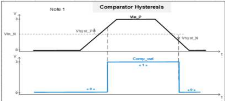
Fig 24. Comparator Hysteresis
