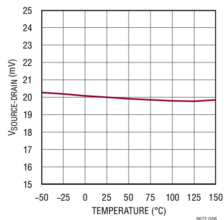
Forward Regulation Voltage
