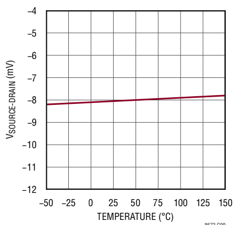
Fast Pull-Down Threshold
