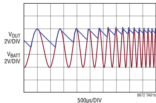
Rectification of Input Ripple
