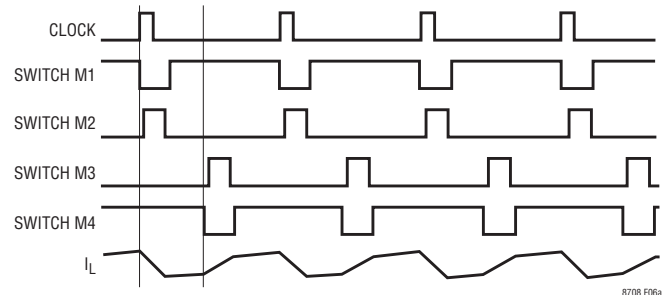
6(a) Buck-Boost Region ( V_{IN} \geq V_{OUT} )
