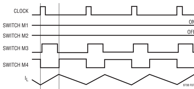
Figure 7. Boost Region ( V_{IN} \ll V_{OUT} )
