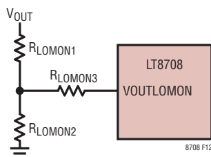
(b) Resistor Divider for VOUTLOMON
