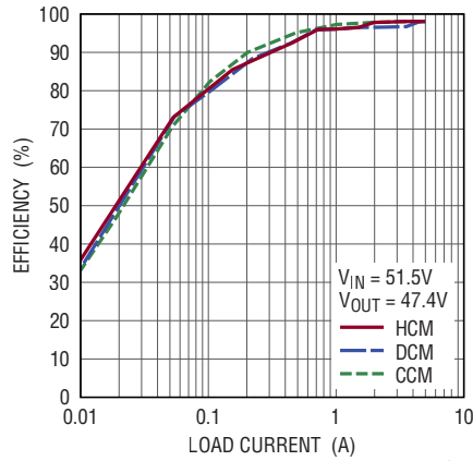
Efficiency vs Output Current (Buck Region – page 59)
