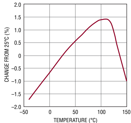
RUN Pin Hysteresis Current vs Temperature
