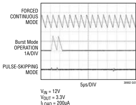
Inductor Current at Light Load
