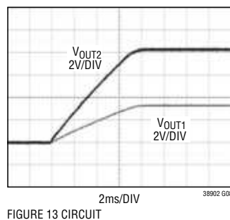
Soft Start-Up
