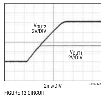
Tracking Start-Up
