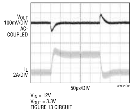
Load Step Forced Continuous Mode
