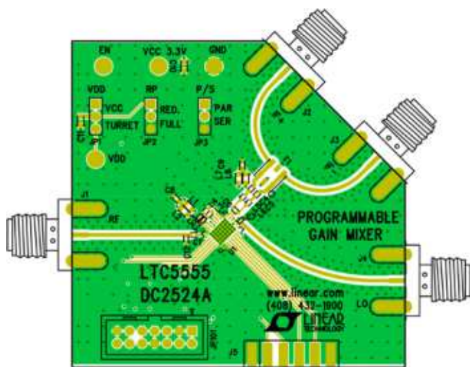
Figure 2. Evaluation Board
