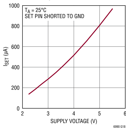
Typical I_{\text{SET}} Current Limit vs V^+
