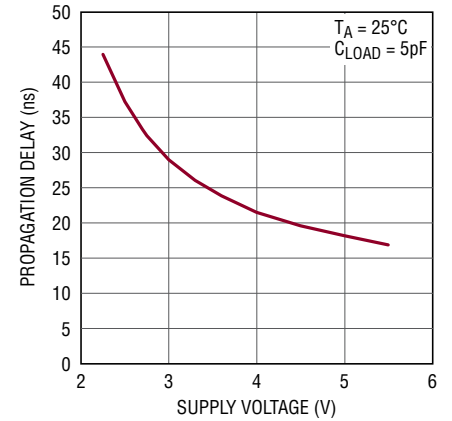
Output Disable Propagation Delay ( t_{\text{PD}} ) vs Supply Voltage
