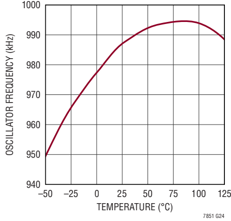
1MHz Preset Frequency vs Temperature
