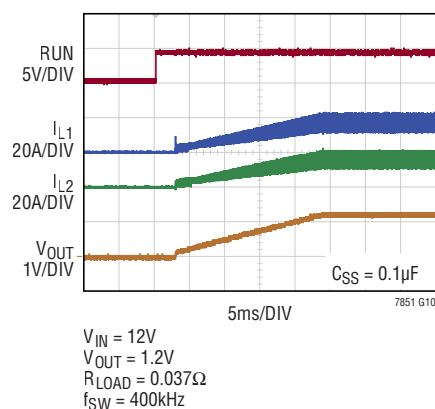
Start-Up Response (2-Phase Using FDMF5820DC DrMOS)
