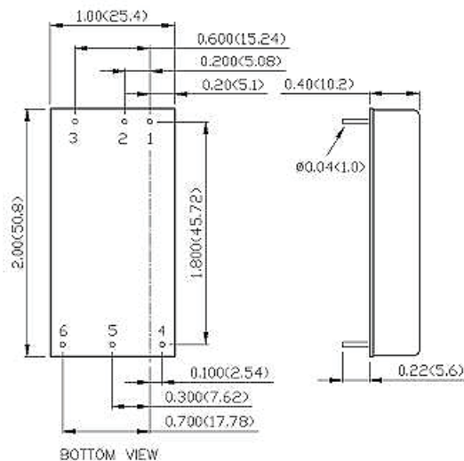
Mechanical Drawing
