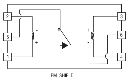
Figure 1 Electrical Configuration
