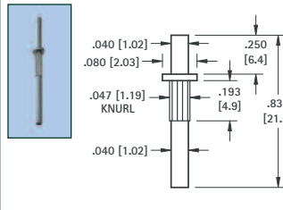
.040 (1.0) KAY PIN - PRESS-FIT
