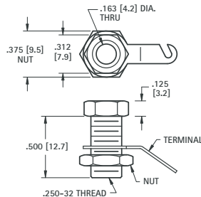
Accepts .175 (4.5) Plug
