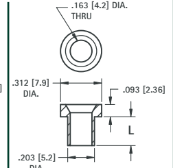
Accepts .175 (4.5) Plug
