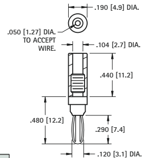
.120 (3.0) Plug
