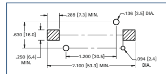
Pad Layout
