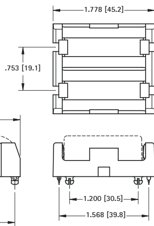
Mounting Detail
