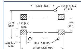
Pad Layout
