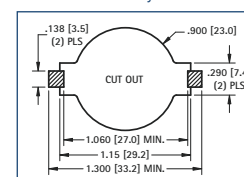
Pad Layout
