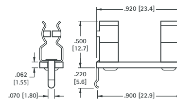
Mounting Detail
