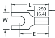
BLOCK SPADE NON-INSULATED
