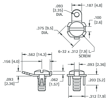
SOLDER TAB
