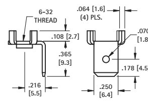
QUICK-FIT
