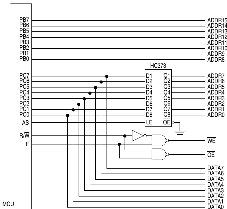
Figure 2-1. Address/Data Demultiplexing
