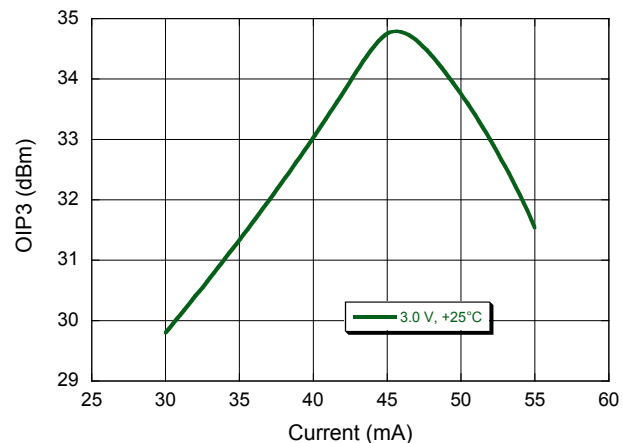
Output IP3 @ 5.5 GHz over bias
