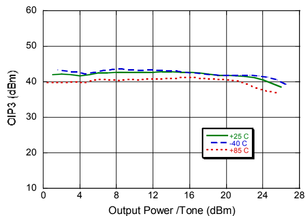
Output IP3
