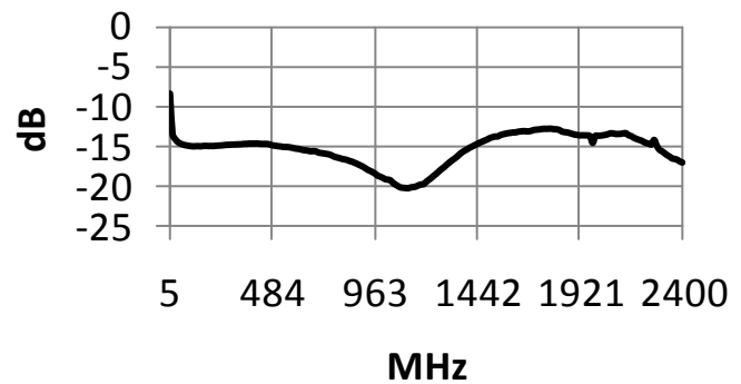
Output Return Loss (pin 2)
