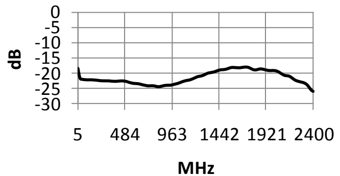
Directivity (pin 1 - pin 4)
