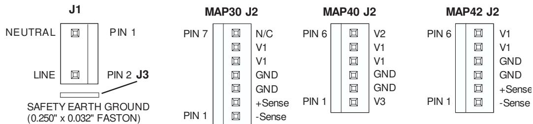
J1/J2 MATES WITH MOLEX (SERIES 2139 or SERIES 41695) .156" (4mm) CENTER CRIMP TERMINAL HOUSING OR EQUIVALENT
