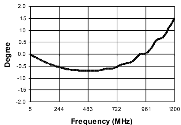
Phase Balance
