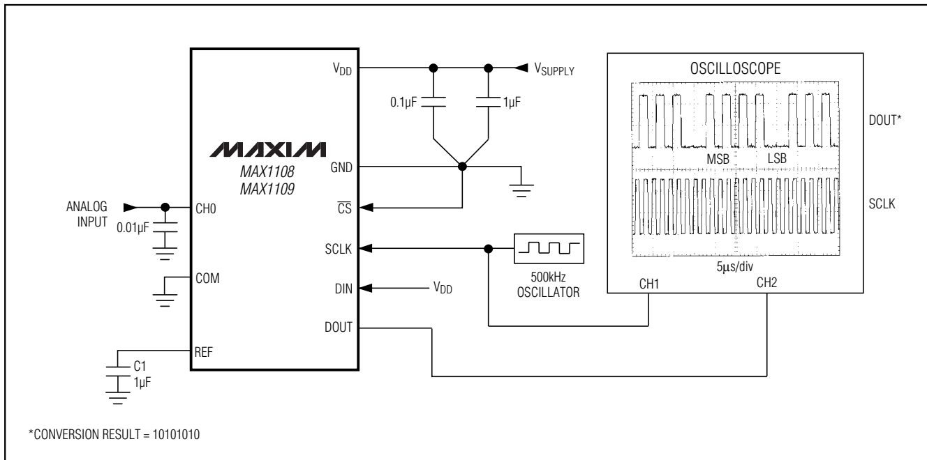
Figure 9. Quick-Look Schematic
