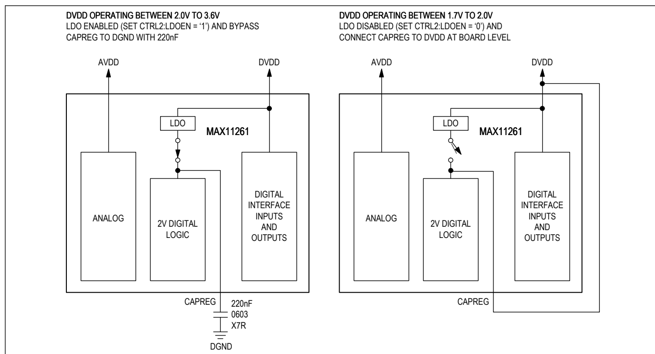
Figure 11. Digital Power Architecture
