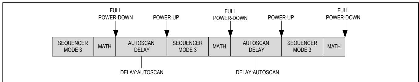
Figure 9. Sequencer Mode 4 Timing Diagram
