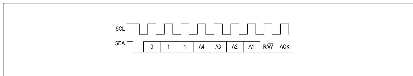
Figure 5. I 2 C Slave Address
