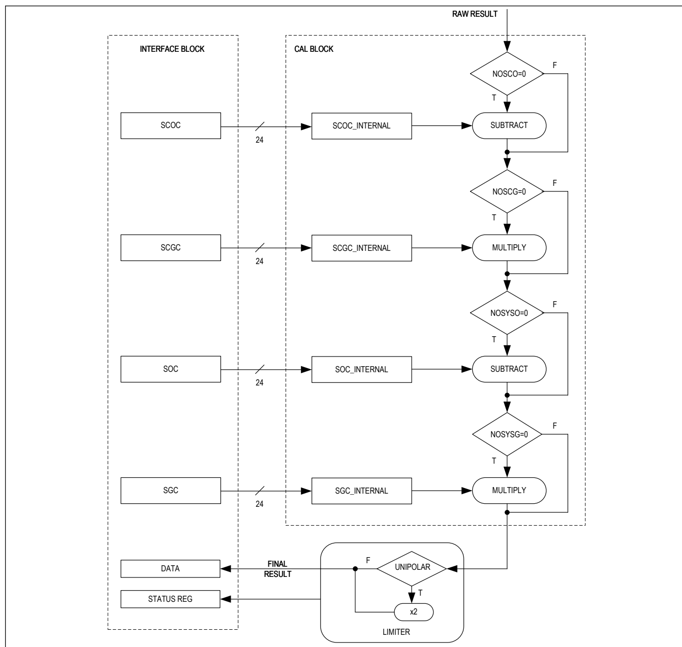
Figure 16. Calibration Flow Diagram
