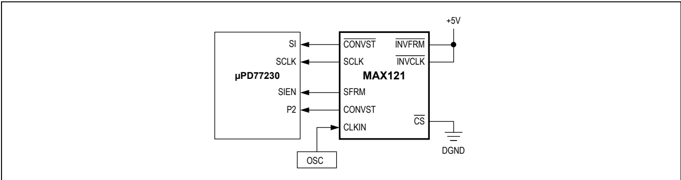
Figure 18. NEC \mu\text{PD77230} Interface Circuit
